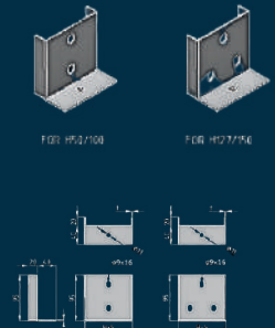
SPLICE PLATE SET FOR STAND
