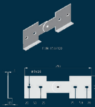
VERTICAL FISH PLATE
