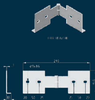
HORIZONTAL FISH PLATE
