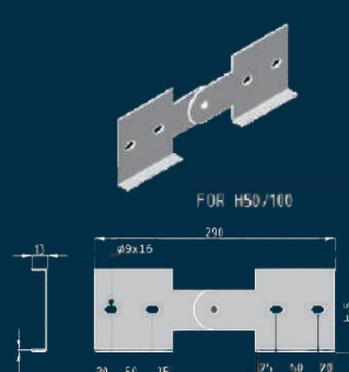
VERTICAL FISH PLATE
