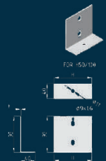
SPLICE PLATE SET FOR STAND
