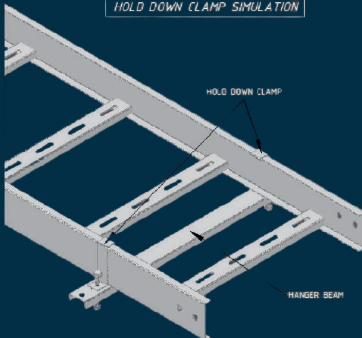
HOLD DOWN CLAMP SIMULATION
