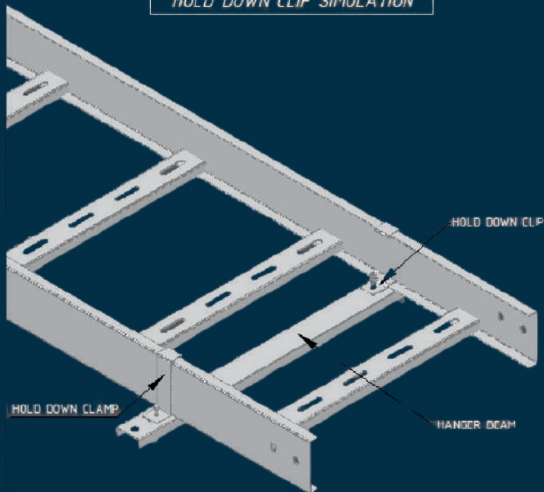
HOLD DOWN CLIP SIMULATION
