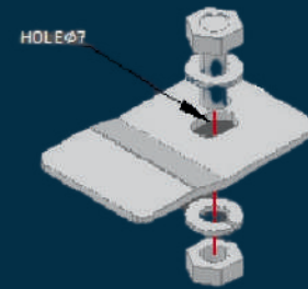
HOLD DOWN CLIP
