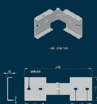
HORIZONTAL FISH PLATE
